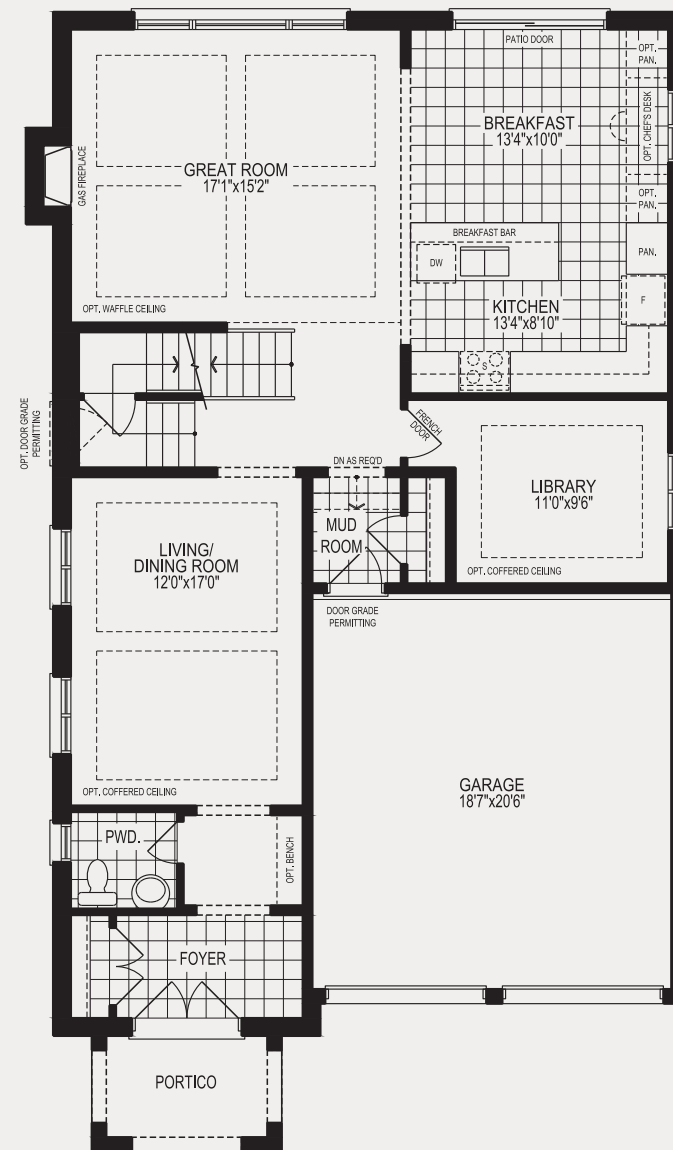
OPT. GROUND FLOOR PLAN A W/LIBRARY
