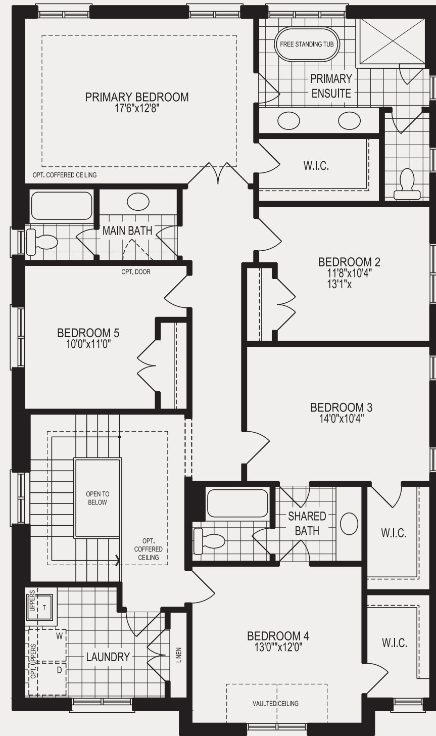
SECOND FLOOR PLAN A
