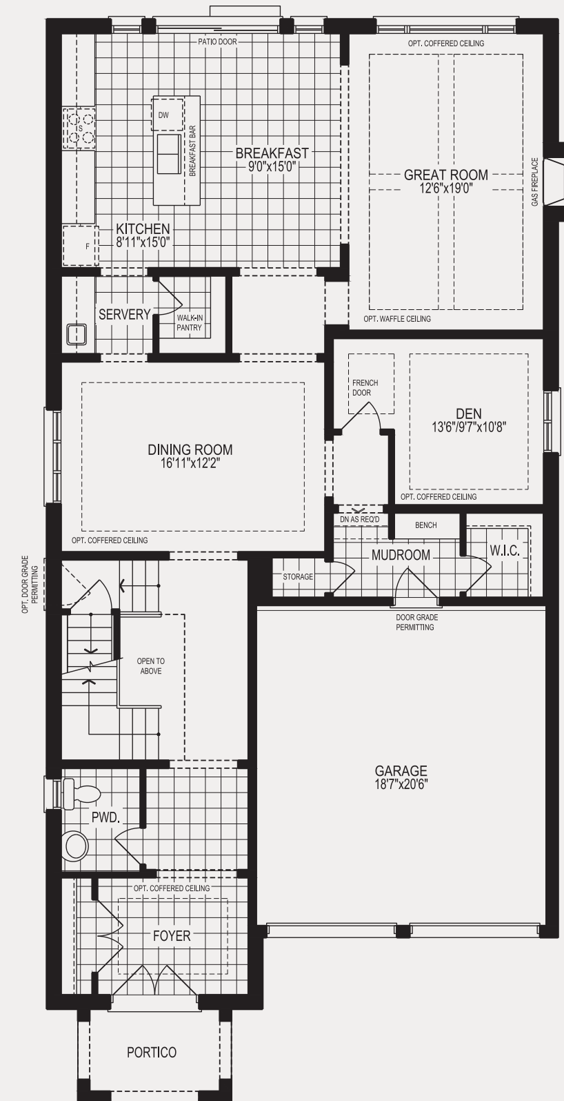
OPT. GROUND FLOOR PLAN A W/DEN
